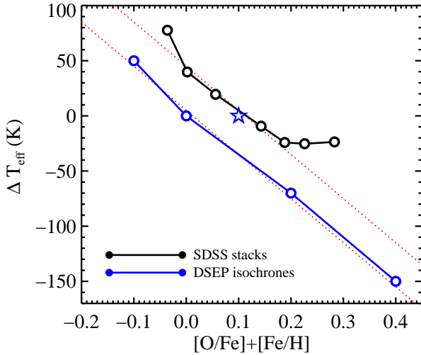
Figure 14. Relation between offset in isochrone T_{\text{eff}} and metal abundance. Results are shown for the stacked SDSS early-type galaxy data and compared to expectations based on theoretical isochrones from the Dartmouth Stellar Evolution Database (DSEP). The theoretical offsets are derived from Figure 5. The star symbol corresponds to the model with [\text{Fe}/\text{H}] = -0.1 and [\alpha/\text{Fe}] = +0.1 and highlights the fact that \Delta T_{\text{eff}} is not a simple function of [\text{Z}/\text{H}] . The dotted lines are offset from each other by 40K. The excellent agreement in the slope between our modeling and the DSEP predictions is a strong indication that our model is able to reliably measure the distribution of T_{\text{eff}} in early-type galaxies.
