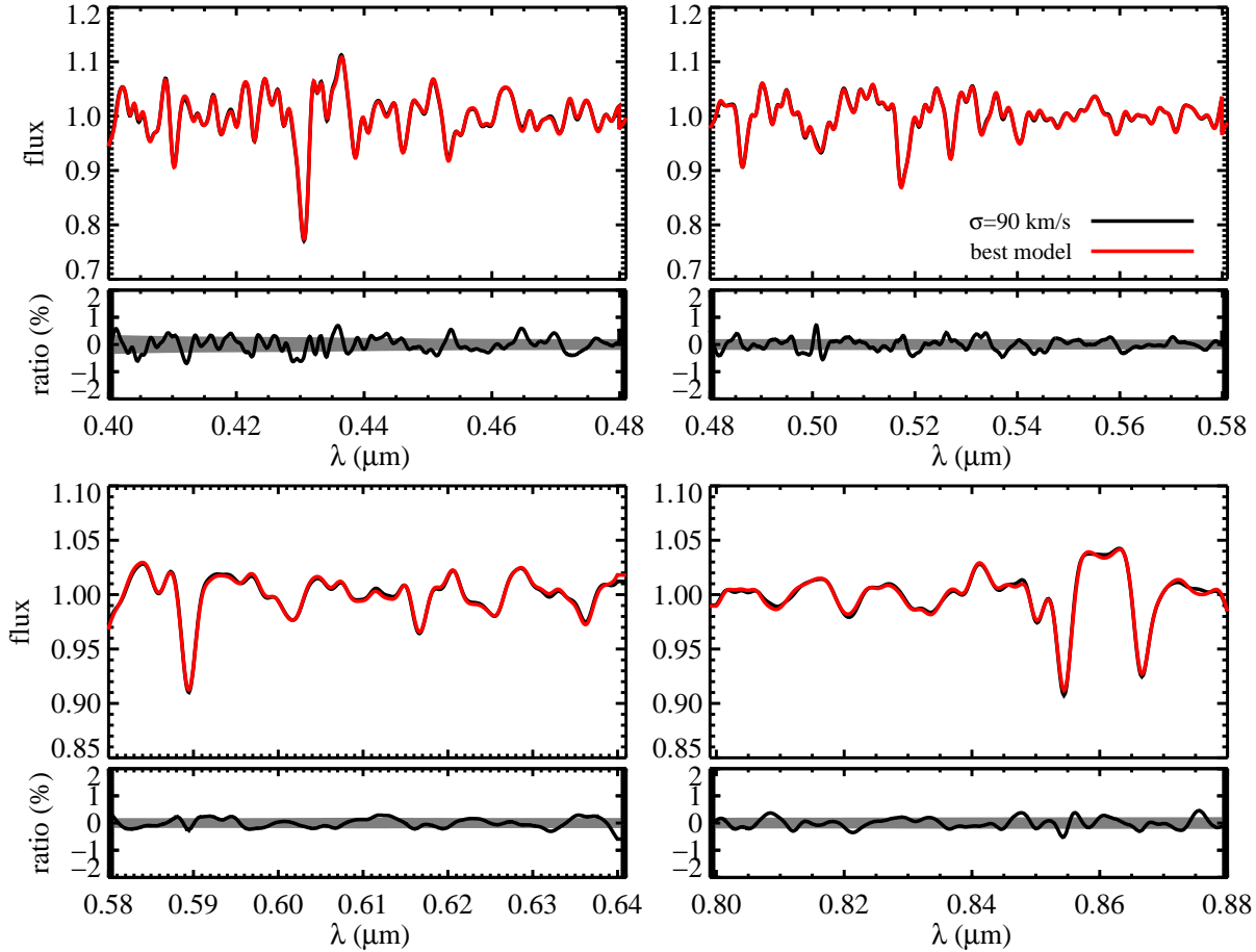
Figure 8. Comparison between the SDSS early-type galaxy stacked spectrum in the lowest velocity dispersion bin (black lines) and the best-fit model (red lines). Within each wavelength range, the top panel shows the continuum-normalized fluxes and the lower panel shows the ratio between data and model. The grey band denotes the 1\sigma error limits of the data. Overall the quality of the fit is excellent.
