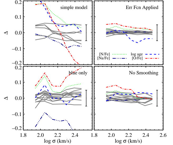
Figure 15. Effect on derived parameters due to varying one or more aspects of our analysis (plotted here as fiducial model minus modified model). All parameters in Table 1 are plotted here (except in the top left panel), but only the most deviant parameters are highlighted. Top Left Panel: Variation between the standard model and a simple model that contains many fewer parameters. Top Right Panel: Variation between the standard model and one in which the mean residuals (averaged over all \sigma bins) are added back into the model. Bottom Left Panel: Variation in parameters when fitting only the blue spectral region ( \lambda < 5800\text{\AA} ). Bottom Right Panel: Variation in parameters when the spectra are not smoothed to a common dispersion of \sigma = 350 \text{ km s}^{-1} . The single error bar in each panel represents an error of \pm 0.05 dex, a value we regard as a plausible upper limit to the systematic errors on the derived parameters.
