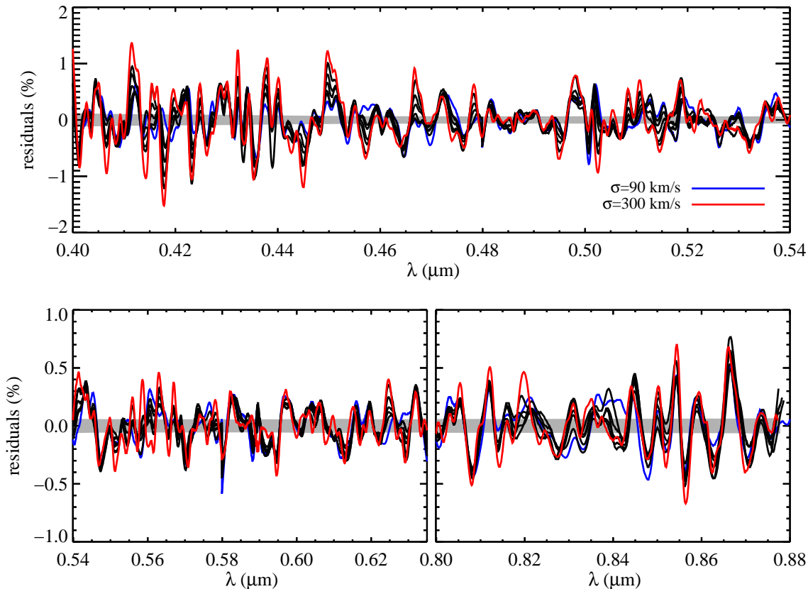
Figure 10. Residuals between the data and best-fit models for all seven stacked early-type galaxy spectra analyzed in this paper. The shaded region marks the noise limit of the middle \sigma bin. In most spectral regions the residuals are constant across the sample, which is an important result because it means that the higher \sigma galaxies, which harbor abundance patterns significantly different from the solar neighborhood, are nearly as well described by our model as the lower \sigma , less metal-enhanced galaxies. In a few spectral regions, e.g., at 0.45\mu\text{m} the residuals correlate with galaxy velocity dispersion, indicating that our model is not capturing the totality of variation in the observed spectra.
