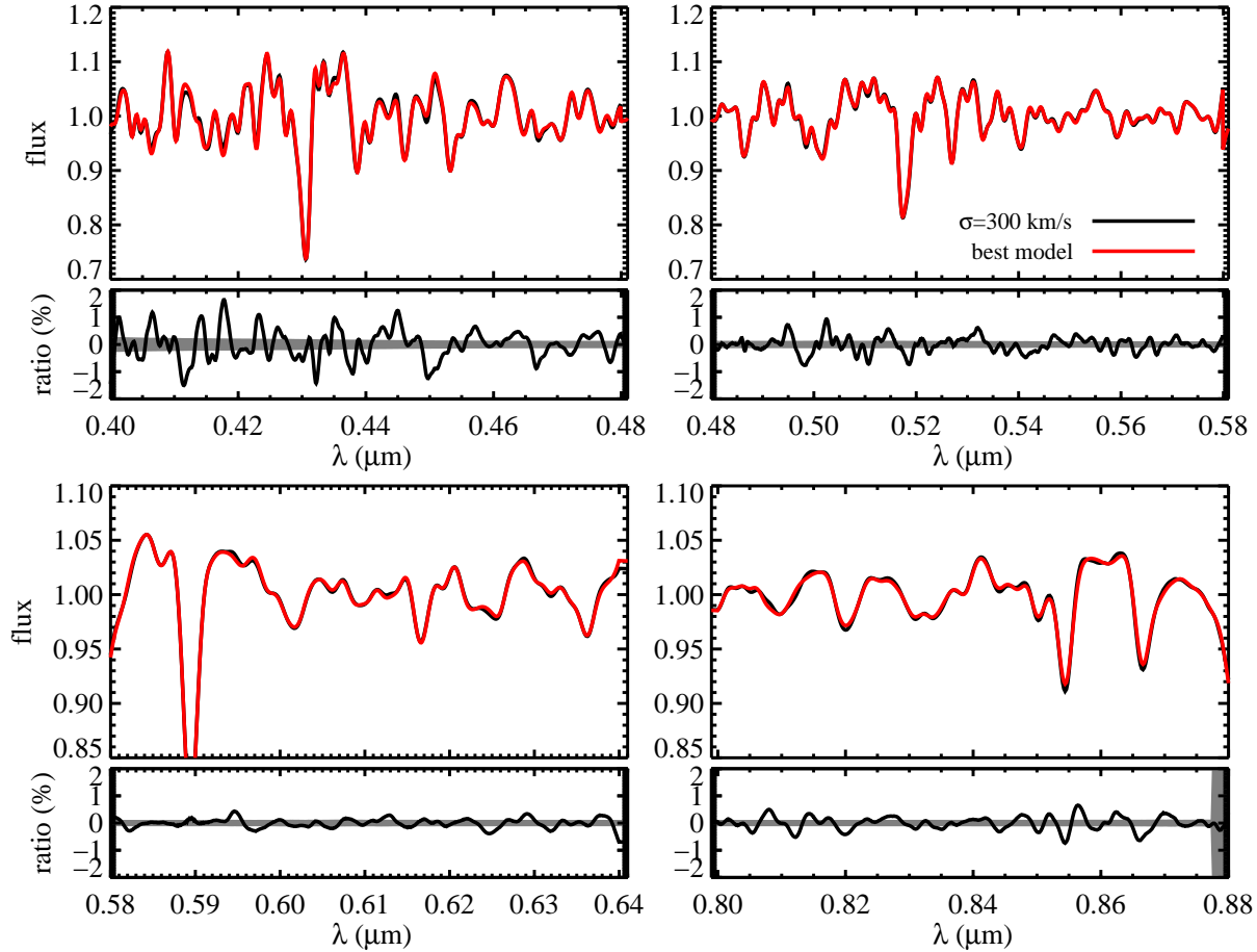
Figure 9. Same as Figure 8, now showing results for the highest velocity dispersion bin. As in Figure 8 the overall quality of the fit is excellent.
