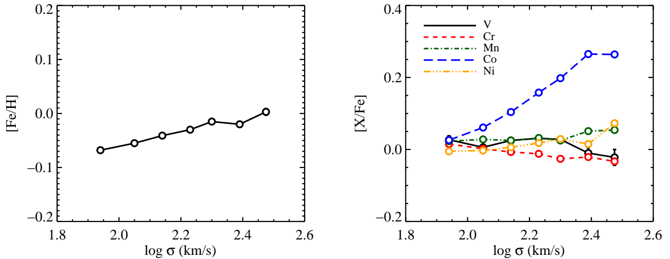
Figure 12. Abundance ratios of the iron peak elements as a function of early-type galaxy velocity dispersion. In most cases the statistical errors are smaller than the symbol sizes. All iron peak elements track Fe except for Co, which seems to track the light \alpha elements O and Mg. Systematic errors are probably < 0.05 dex (see Section 5.4).
