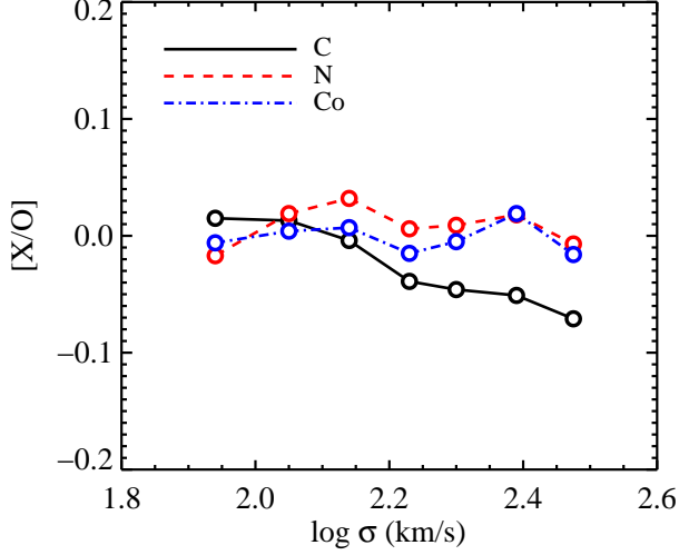
Figure 13. Abundance ratios between C, N, Co, and O as a function of early-type galaxy velocity dispersion. All of these elements seem to track each other very closely, especially N, O, and Co. Systematic errors are probably < 0.05 dex (see Section 5.4).
