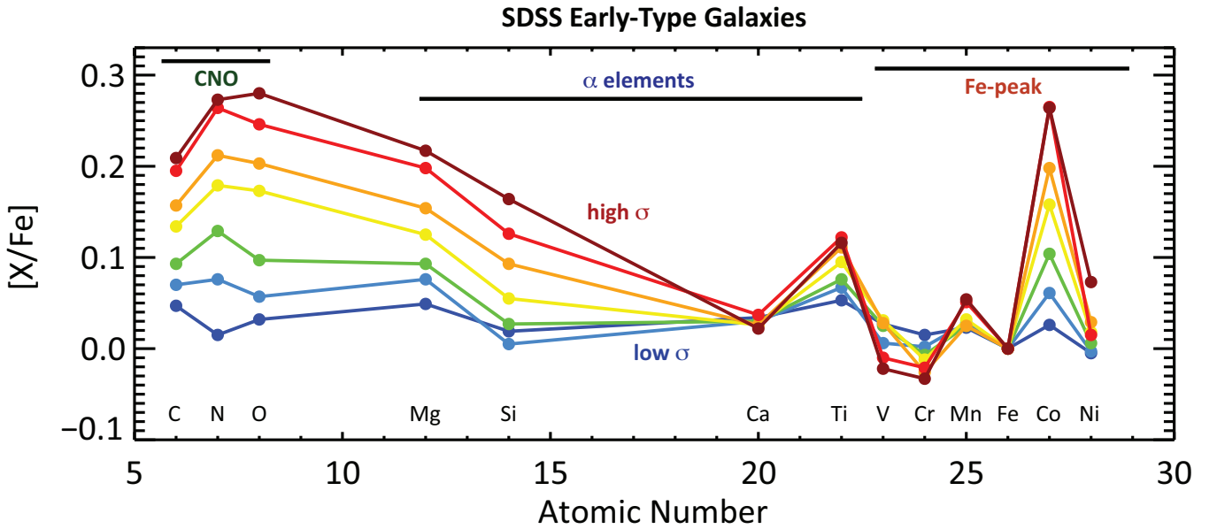
Figure 17. Summary of the abundance trends derived herein from stacked spectra of SDSS early-type galaxies. The sample spans a range in velocity dispersion from \sigma = 90 \text{ km s}^{-1} to \sigma = 300 \text{ km s}^{-1} . The results for Na are omitted from this summary diagram, though we note that [\text{Na}/\text{Fe}] varies from -0.16 to +0.43 from low to high \sigma .
