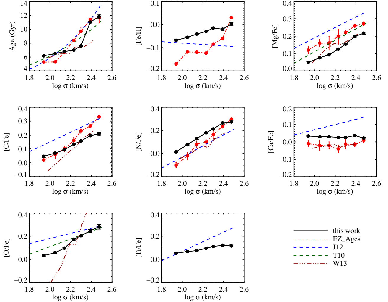
Figure 16. Comparison between different techniques for estimating ages and elemental abundances. Our results are compared to techniques that rely on Lick index fitting, including Graves & Schiavon (2008, EZ_Ages), Thomas et al. (2010, T10), Johansson et al. (2012, J12), and Worthey et al. (2013, W13). The EZ_Ages results are based on modeling the exact same stacked spectra as used herein, while the W13 results are based on similar but not identical stacks, while the T10 and J12 results are linear fits to results obtained for \sim 4000 SDSS early-type galaxies with light-weighted ages greater than 2.5 Gyr. Note that T10 derive a single [\alpha/\text{Fe}] ratio, which we plot in both the [Mg/Fe] and [O/Fe] panels, as it is not entirely clear which element their [\alpha/\text{Fe}] parameter is most sensitive to. Qualitatively the derived trends agree well between various methods/groups, although quantitative differences are clearly evident.
