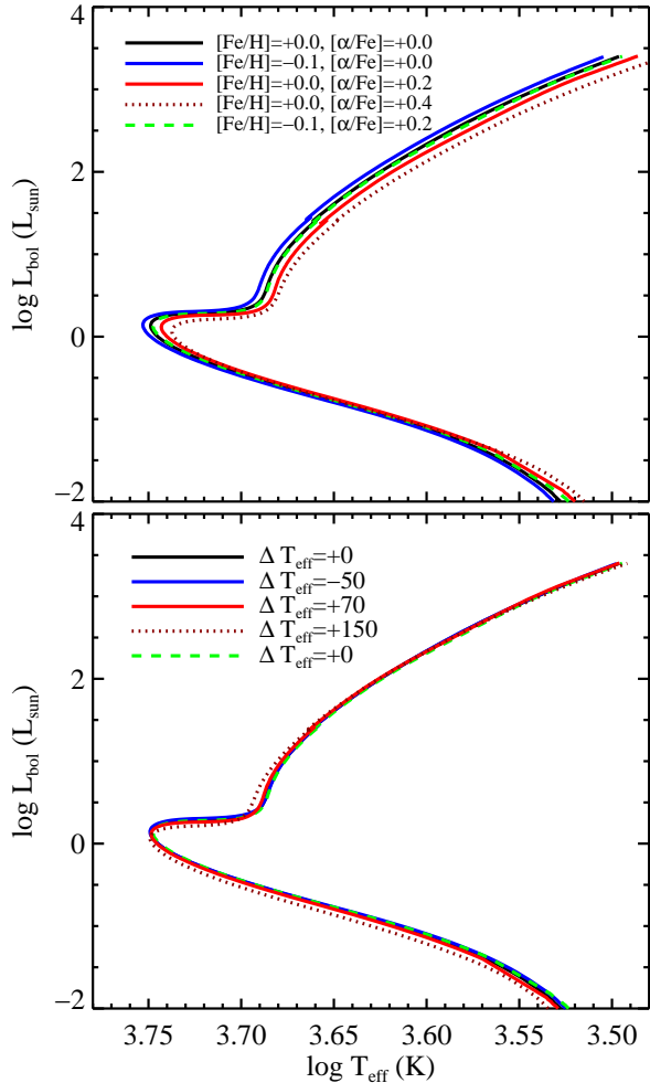
Figure 5. Isochrones at 13.4 Gyr from the Dartmouth Stellar Evolution Database (DSEP) for a variety of chemical compositions. Top panel: Isochrones for a range in compositions approximately spanned by the early-type galaxies in our sample. The case with [\text{Fe}/\text{H}] = 0.0 and [\alpha/\text{Fe}] = +0.4 is extreme, as no galaxies in the sample have such large \alpha enhancements. Notice that the isochrone with [\text{Fe}/\text{H}] = -0.1 and [\alpha/\text{Fe}] = 0.2 is almost identical to the solar metallicity isochrone. Bottom panel: Same isochrones as in the top panel, with a constant shift in T_{\text{eff}} applied to the entire isochrone (the shift applied is shown in the legend). For the modest range in chemical compositions probed by our sample, the expected effective temperatures of the stars can therefore be well-approximated by a solar metallicity model with a single additional free parameter describing the offset in T_{\text{eff}} .
