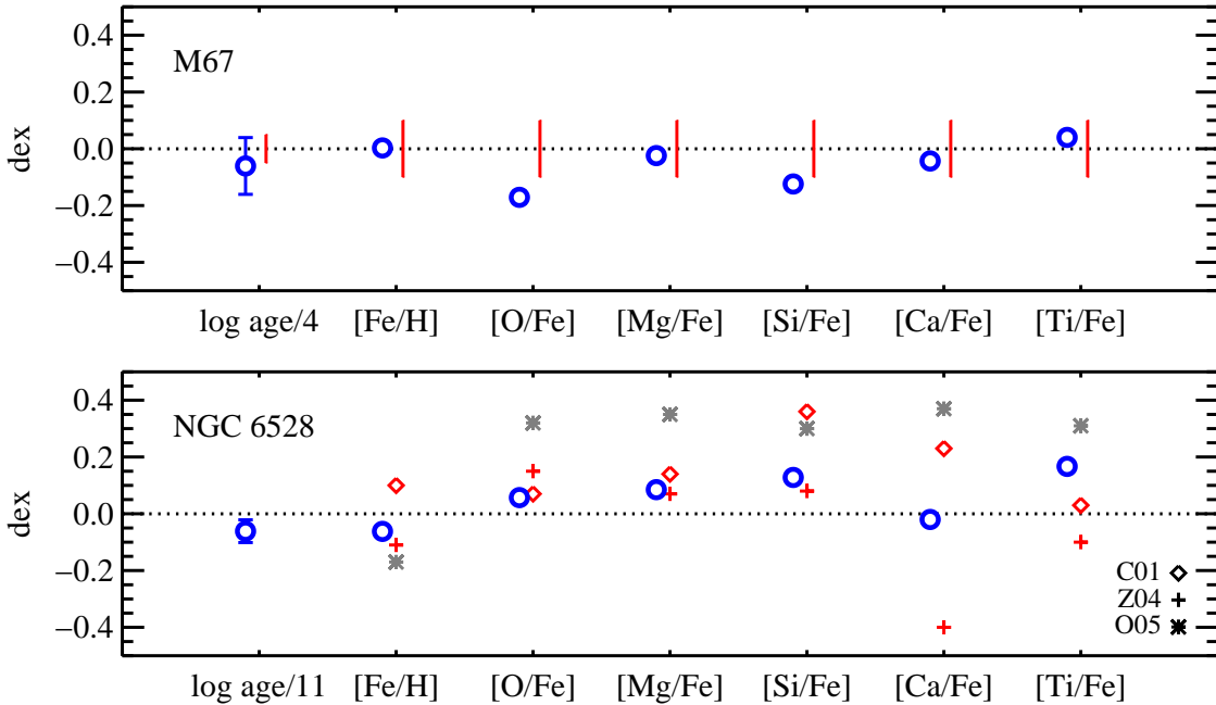
Figure 7. Best-fit parameters for the star clusters M67 (top panel) and NGC 6528 (bottom panel). Results from our full-spectrum fitting of the integrated light (open blue circles) are compared to literature values based on high resolution spectra of individual member stars (red lines and symbols). Fiducial ages for M67 and NGC6528 are taken to be 4 and 11 Gyr, respectively, based on isochrone fitting to their CMDs. Abundance patterns for NGC 6528 are from Carretta et al. (2001, C01), Zoccali et al. (2004, Z04), and Origlia et al. (2005, O05). For M67 we adopt a fiducial abundance pattern of 0.0 \pm 0.1 (roughly 1\sigma errors Tautvaišienė et al. 2000; Shetrone & Sandquist 2000). Overall the agreement between our model predictions and the literature values is good, although the large variation in the literature determination of many of the elemental abundances for NGC 6528 prohibits a more definitive test of our model.
