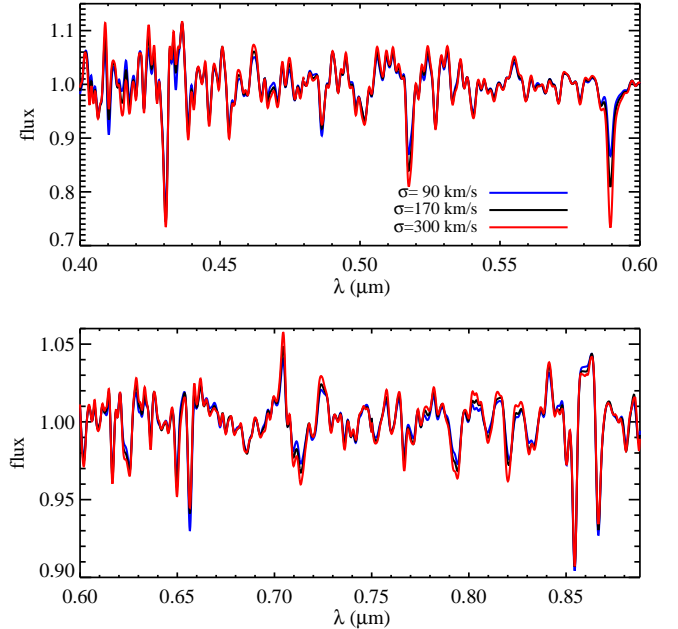
Figure 6. Continuum-normalized stacked spectra of SDSS early-type galaxies in three velocity dispersion bins.
