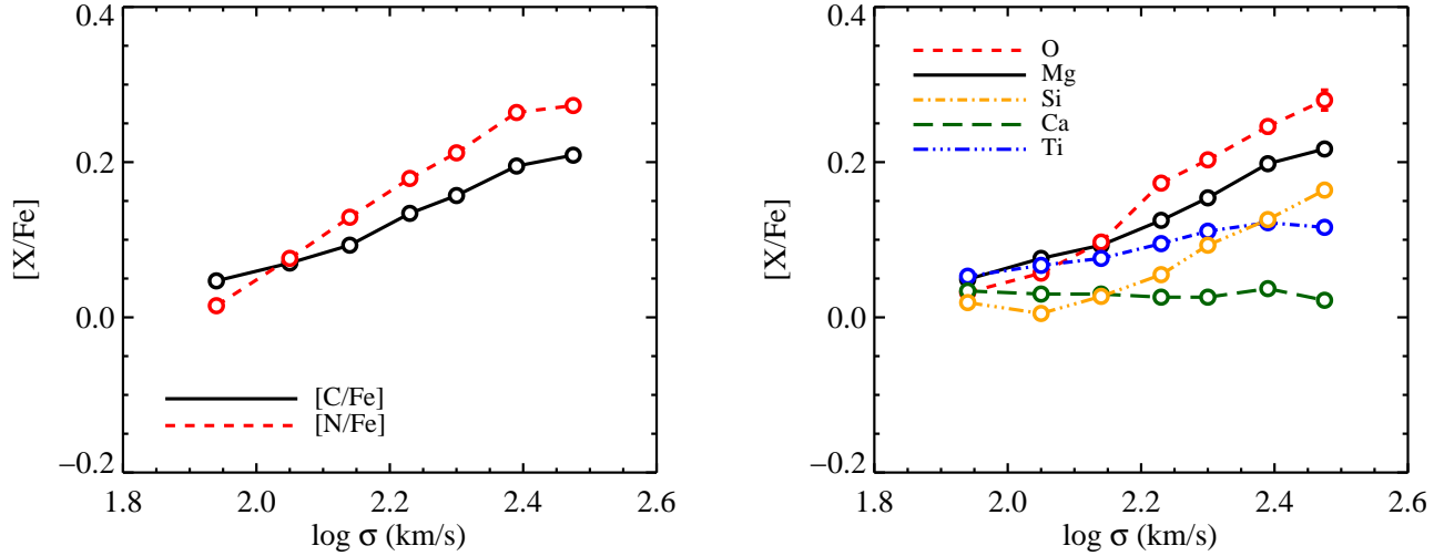
Figure 11. Abundance ratios of C, N, and the \alpha elements as a function of early-type galaxy velocity dispersion. In most cases the statistical errors are smaller than the symbol sizes. C, N, O, and Mg all seem to track each other fairly closely, while the heavier \alpha elements Si, Ca, and Ti show weaker trends with \sigma . Ca clearly tracks Fe instead of O. Systematic errors are probably < 0.05 dex (see Section 5.4).
